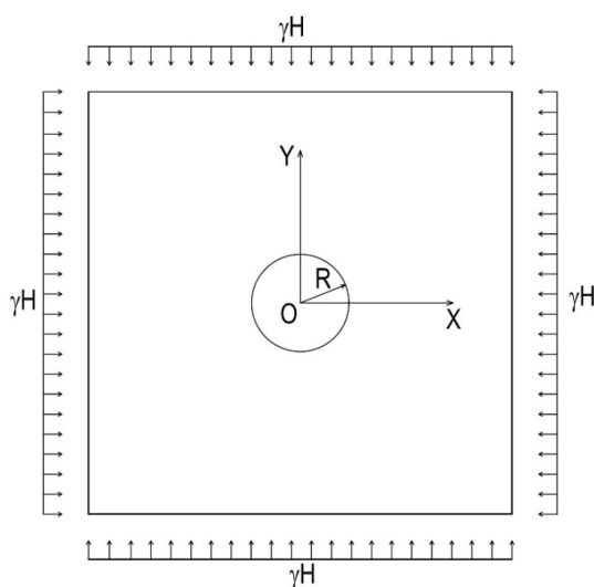
Figure 1 – Calculation scheme
